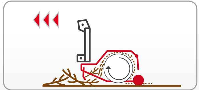
Closed rear hood: to smoothly mulch prunings and branches
